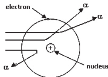
Fig. Scattering of alpha particle
