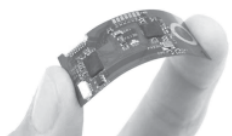
IMEC's flexible wireless monitoring system for vital body parameters with embedded microcontroller chip.
