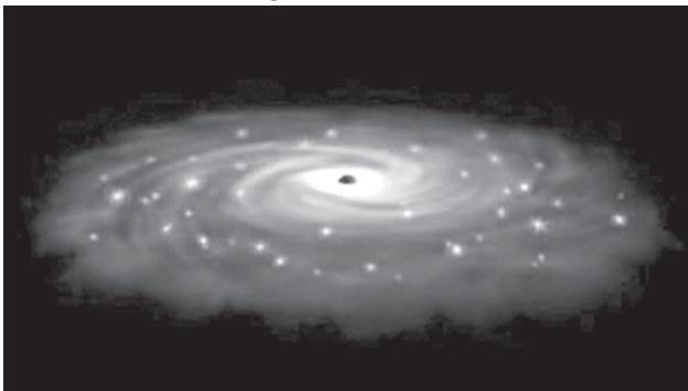
The ring of stars circling Sagittarius A*, the Milky Way's central black hole, shows a combination of infrared and X-ray observations indicating that a surplus of massive stars has formed from a large disk of gas around the black hole in this artist's concept released on 30 Oct, 2005.—INTERNET
