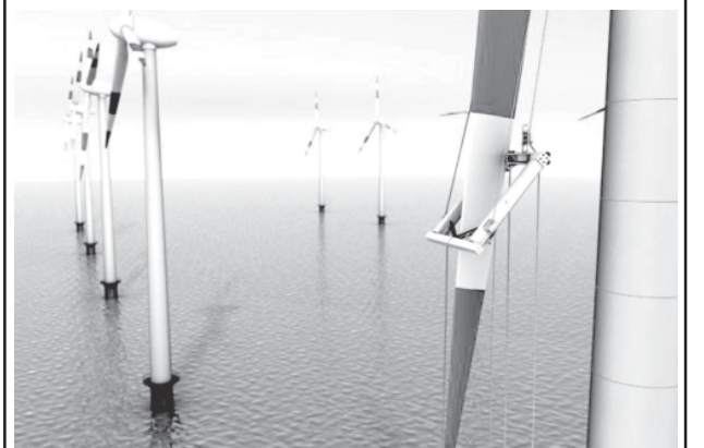
A robot inspects a wind energy converter's rotor blades for possible damage.
