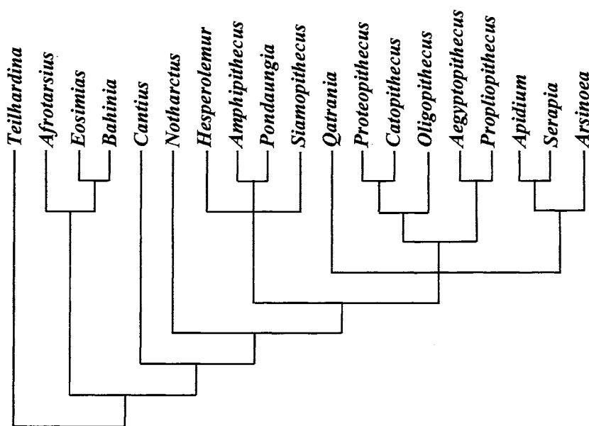
FIG. 25 — Fifty-percent-majority-rule consensus phylogenetic tree based on a branch and bound analysis of 19 taxa and 22 dental, cranial, and postcranial characters (see Tables 5 and 6). Results based on 36 equally parsimonious trees of 64 steps. CI = 0.688, RI = 0.756, HI = 0.312 (PAUP 4.1).
