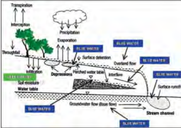
ပုံ(၁၀) Hydrological Cycle for Basin Scale (FAO, 2013)
