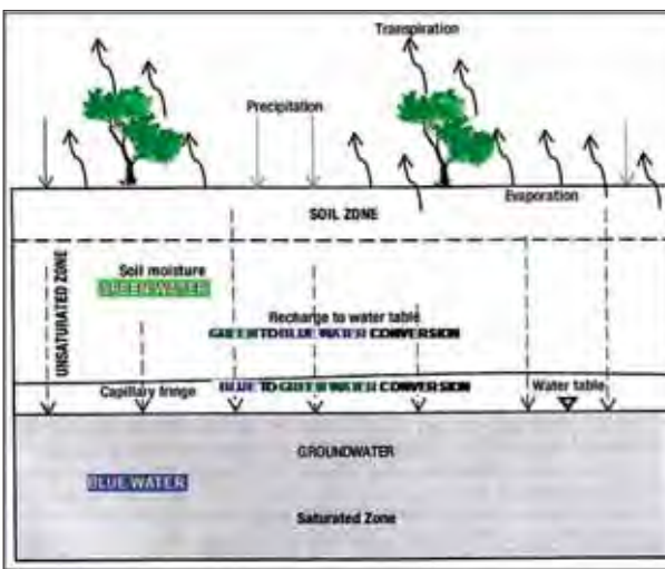
ပုံ(၁၁) H ydrological Process within a Vadose Zone (USES, 2013)
