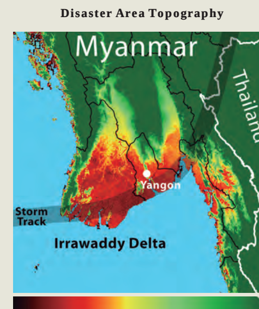
Figure 8.2. Storm track and elevation of regions of Myanmar hit by Cyclone Nargis in 2008. Source: Robert A. Rohde, elevation data based on NASA SRTM.
