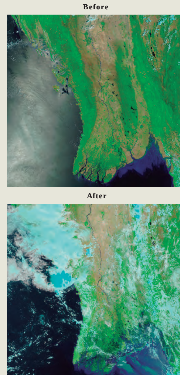
Figure 8.1. NASA's Terra satellite image of the Myanmar coast on April 15th, 2008 (top), before Tropical Cyclone Nargis flooded the region, compared to NASA's Terra Satellite image of the coastal region on May 5th, 2008 (bottom), showing the devastation of flooding caused by Tropical Cyclone Nargis. Source: NASA/MODIS Rapid Response Team
