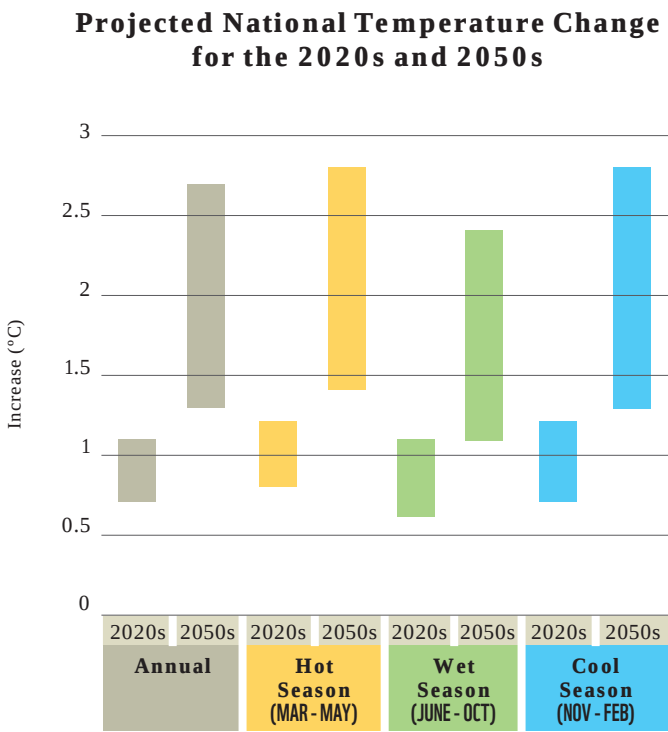
Figure 4.2. Range of average annual temperature change (low estimate to high estimate) relative to the 1980–2005 base period. Note: Data source for temperature projections is NASA Earth Exchange Global Daily Downscaled Projections (NASA NEX GDDP, 2015).
