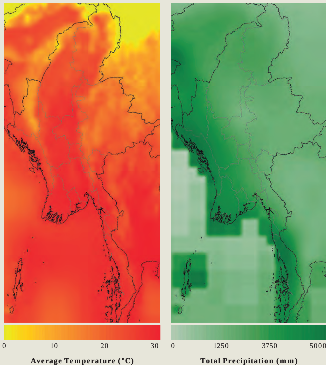
Figure 2.1. Baseline annual average temperature climatology across Myanmar (1980-2005) from climate model outputs.
