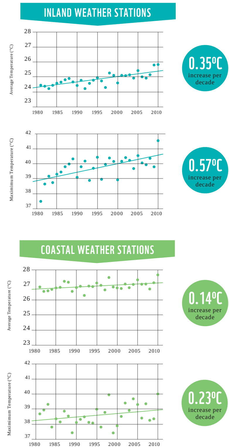
Figure 3.1. Trends in daily average and daily maximum temperatures on average across 9 inland (blue) and 10 coastal (green) weather stations, 1981-2010. Weather station data provided by DMH (2015).
