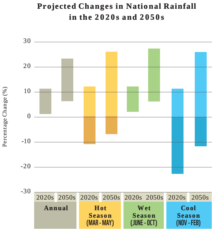
Figure 5.2. Range of average annual rainfall percentage change (low estimate to high estimate) relative to the 1980–2005 base period. Note: Data source for precipitation projections is NASA Earth Exchange Global Daily Downscaled Projections (NASA NEX GDDP, 2015).
