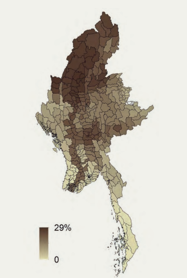
Figure 1.1. Potential change in sediment retention under high climate change scenario RCP 8.5. Source: Mandle et al. , 2016.
