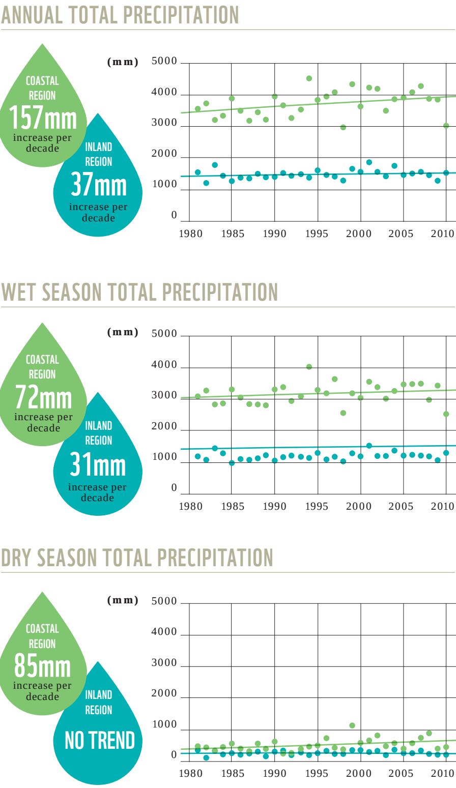
Figure 3.2. Trends in total annual [top], wet season (June to October) [center], and dry season (November to May) [bottom] precipitation for 10 coastal (green) and 9 inland (blue) weather stations, 1981-2010. Weather station data provided by DMH (2015).
