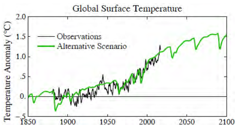
Figure A12. Simulated global temperature with historical climate forcings to 2000 followed by the alternative scenario. Historical climate forcings are discussed in the main text.
