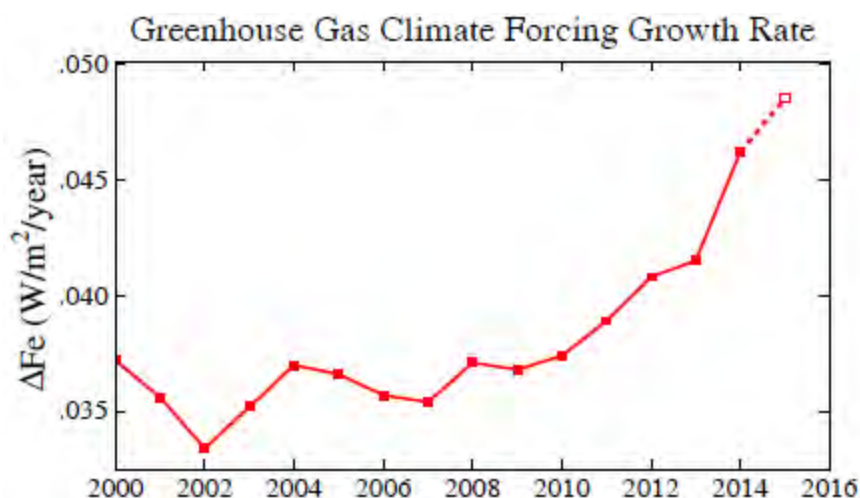
Figure 14. Recent growth rate of total GHG effective climate forcing; points are 5-year running means, except 2015 point is a 3-year mean. See Fig. 8 for individual gases.
