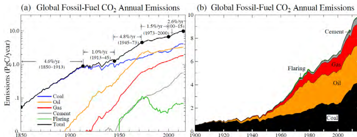
Figure A1. CO 2 emissions from fossil fuels and cement use based on Boden et al. (2017) through 2014, extended using BP (2016) energy consumption data. (a) is log scale and (b) is linear. Growth rates r in (a) for an n -year interval are from (1+r)^n with end values being 3-year means to minimize noise.
