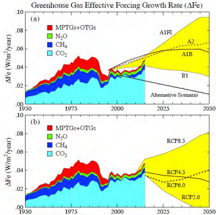
Figure 8. GHG climate forcing annual growth rate ( \Delta Fe ) with historical data being 5-year running means, except 2015 is a 3-year mean. (a) includes scenarios used in IPCC AR3 and AR4 reports, and (b) has AR5 scenarios. GHG amounts are from NOAA/ESRL Global Monitoring Division. O_3 changes are not fully included, as they are not well-measured, but its tropospheric changes are partially included via the effective CH_4 forcing. Effective climate forcing ( Fe ), MPTGs and OTGs are defined in Fig. 4 caption.
