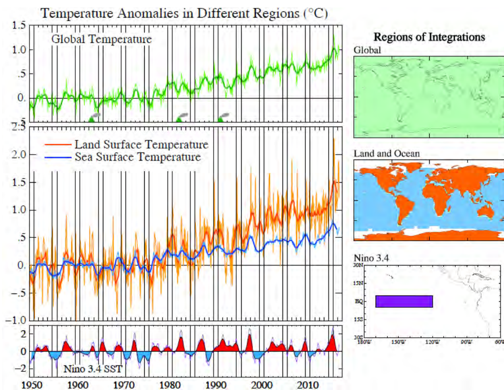
Figure A3a. Monthly (thin lines) and 12-month running mean (thick lines or filled colors for Niño 3.4) global, global land, sea surface, and Niño 3.4 temperatures. Temperatures are relative to 1951-1980 base period for the current GISTEMP analysis, which uses NOAA ERSST.v4 for sea surface temperature.
