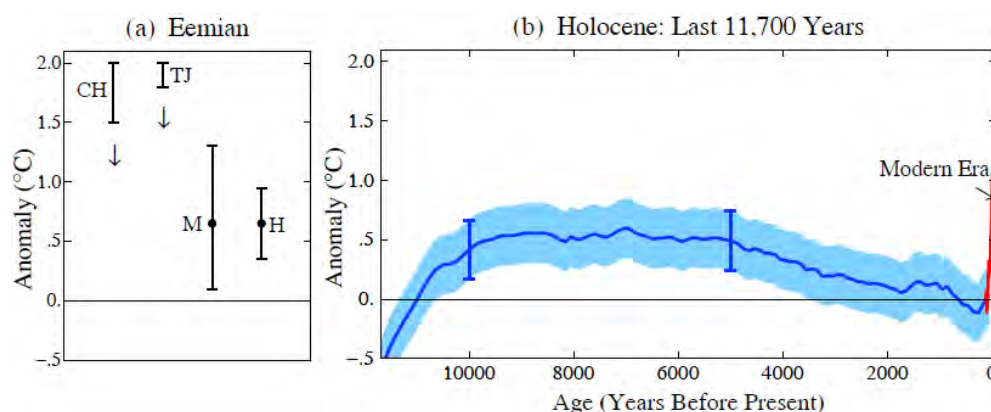
Figure 3. Estimated average global temperature for (a) last interglacial (Eemian) period (Clark and Huybers, 2009; Turney and Jones, 2010; McKay et al., 2011; Hoffman et al, 2017), (b) centennially-smoothed Holocene (Marcott et al., 2013) temperature and the 11-year mean of modern data (Fig. 2), as anomalies relative to 1880-1920. Vertical downward arrows indicate likely overestimates (see text).
