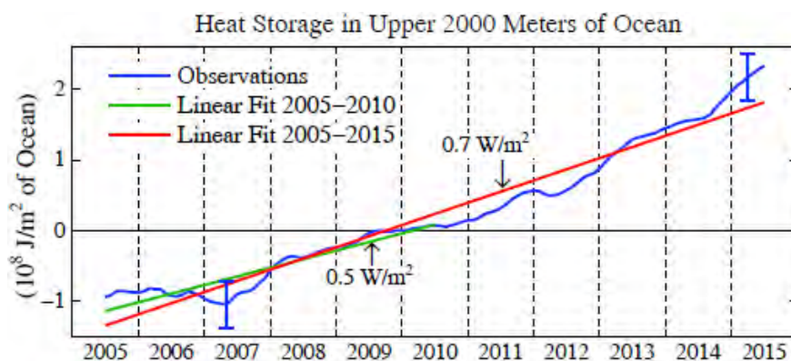
Figure 5. Ocean heat uptake in upper 2 km of ocean during 11 years 2005-2015 using analysis method of von Schuckmann and LeTraon (2011). Heat uptake in \text{W/m}^2 (0.5 and 0.7) refer to global (ocean + land) area, i.e., it is the contribution of the upper ocean to the heat uptake averaged over the entire planet.
