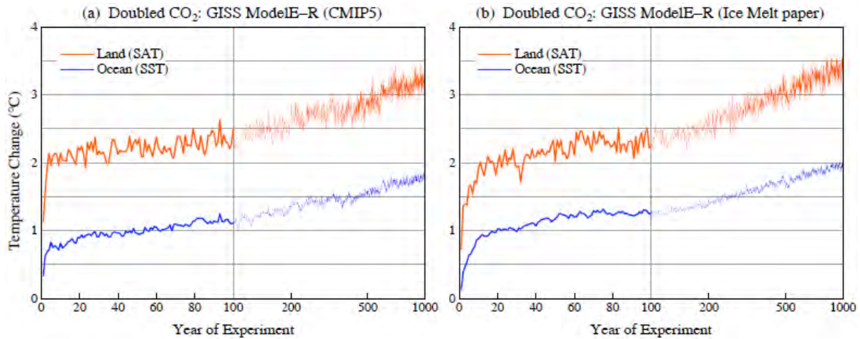
Figure A6. 1000-year temperature response in two versions of GISS ModelE-R. (a) version used for CMIP5 simulations (Schmidt et al. 2014), which has higher resolution (40-layer atmosphere at 2^\circ \times 2.5^\circ , 32-layer ocean at 1^\circ \times 1.25^\circ ), (b) version used by Hansen et al. (2016), which has coarse resolution (20-layer atmosphere at 4^\circ \times 5^\circ , 12-layer ocean at 4^\circ \times 5^\circ ) and includes two significant improvements to small scale ocean mixing, cf. section 3.2 of Hansen et al. (2016).
