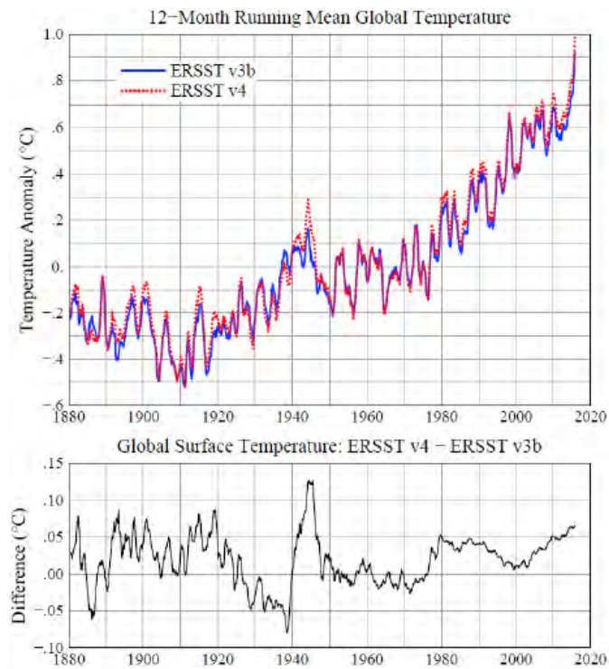
Figure A3b. Global surface temperature relative to 1951-1980 in the GISTEMP analysis, comparing the current analysis using NOAA ERSST.v4 for sea surface temperature with results using ERSST.v3b.
