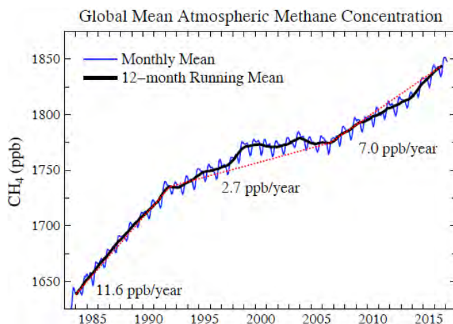
Figure 7. Global CH 4 from Dlugokencky (2016), NOAA/ESRL ( www.esrl.noaa.gov/gmd/ccgg/trends_ch4/ ). End months for three indicated slopes are January 1984, May 1992, August 2006, and February 2017.
