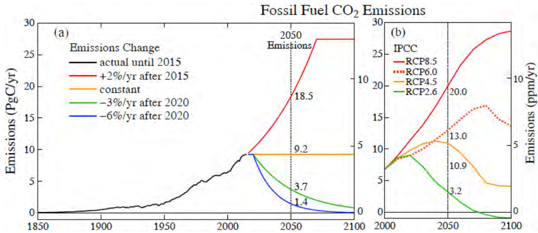
Figure 9. Fossil fuel emission scenarios. (a) Scenarios with simple specified rates of emission increase or decrease. (b) IPCC (2013) RCP scenarios. Note: 1 ppm atmospheric CO 2 is ~2.12 GtC.
