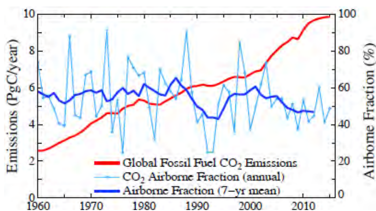
Figure A8. Fossil fuel CO 2 emissions (left scale) and airborne fraction, i.e., the ratio of observed atmospheric CO 2 increase to fossil fuel CO 2 emissions.
