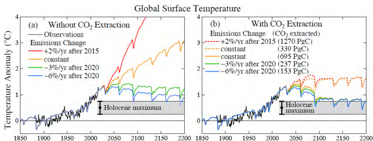
Figure 12. Simulated global temperature for Fig. 11 forcings. Observations as in Fig. 2. Temperature zero-point is the 1880-1920 mean temperature for both observations and model. Gray area is 2\sigma (95% confidence) range for centennially-smoothed Holocene maximum, but there is further uncertainty about the magnitude of the Holocene maximum, as noted in the text and discussed by Liu et al. (2014).
