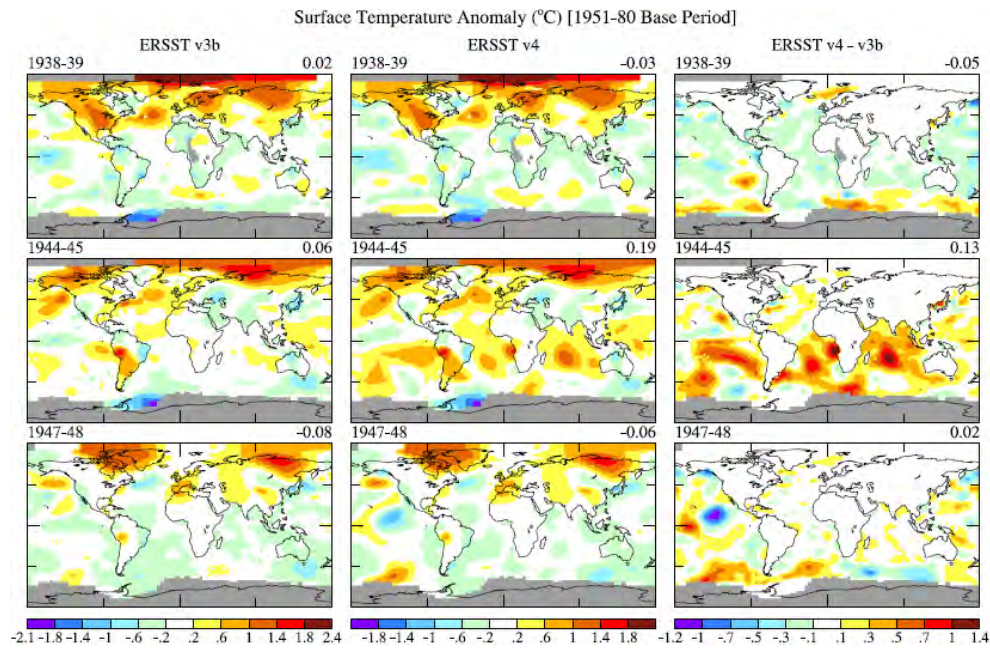
Figure A3c. Temperature anomalies in three periods relative to 1951-1980 comparing results obtained using ERSST.v3b (left column), ERSST.v4 (center column), and their difference (right column).
