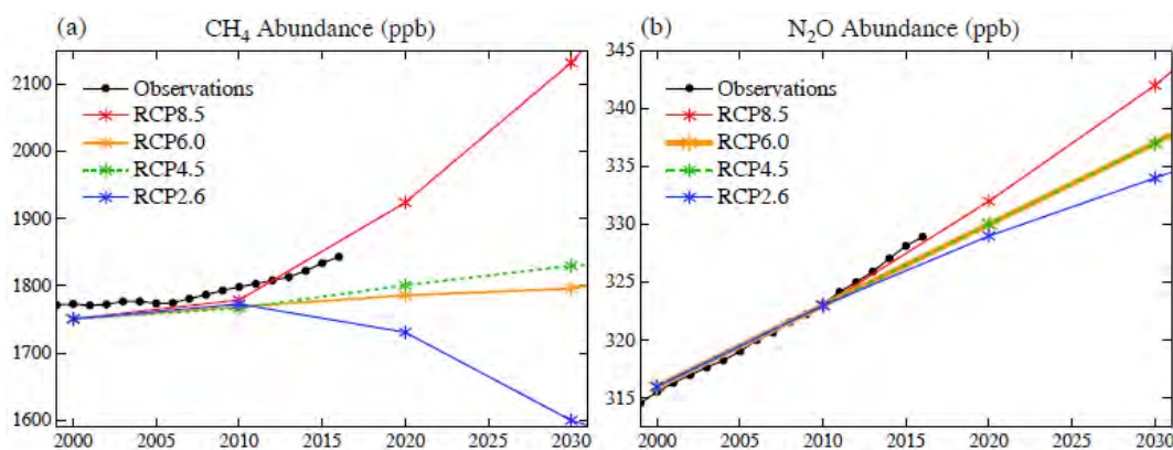
Figure A13. Comparison of observed CH 4 and N 2 O amounts with RCP scenarios. RCP 6.0 and 4.5 scenarios for N 2 O overlap. Observations are from NOAA/ESRL Global Monitoring Division. Natural sources and feedbacks not included in RCP scenarios may contribute to observed growth (see discussion).
