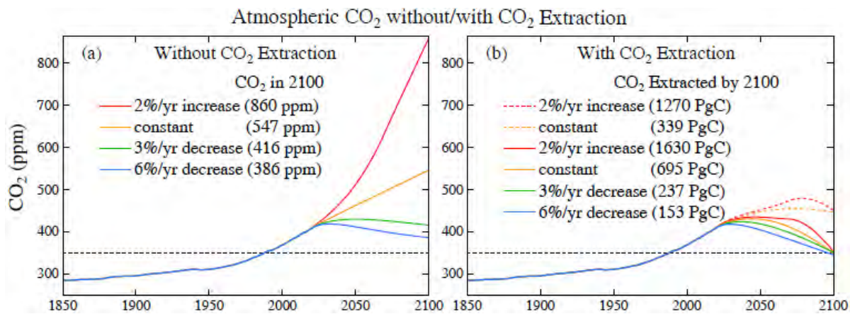
Figure 10. (a) Atmospheric CO 2 for Fig. 9a emission scenarios. (b) Atmospheric CO 2 including effect of CO 2 extraction that increases linearly after 2020 (after 2015 in +2%/year case).
