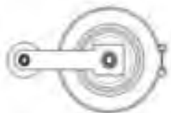
FIG. 6 - Bottom Plan View
