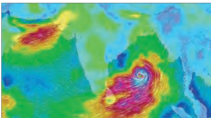
Pictorial description of possible cyclonic storm.
