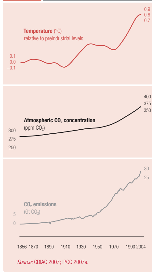
Figure 1.1 Rising CO 2 emissions are pushing up stocks and increasing temperature
