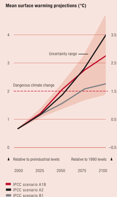
Figure 1.2 Global temperature forecast: three IPCC scenarios
