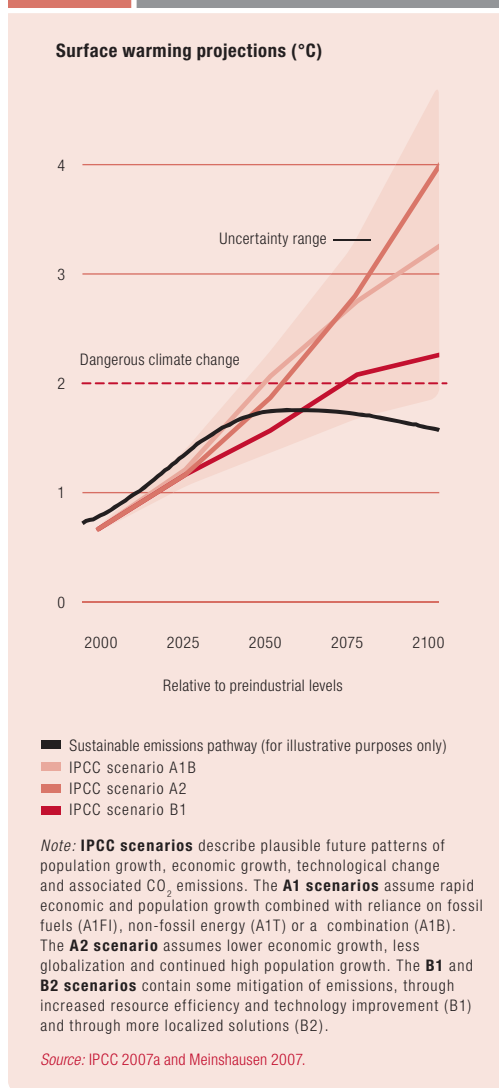
Figure 1.13 Stringent mitigation does not deliver early results
