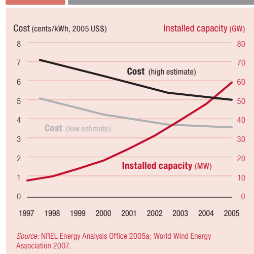
Figure 3.4 Wind power in the US—capacity is increasing and costs are falling
