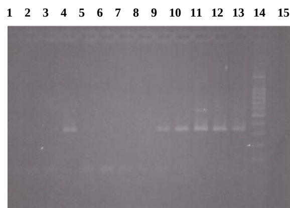
Fig.1. Nested PCR for amplification of 347bp DNA of M. leprae from biopsy tissue. Lane 1, negative control, lane 2, 3, 5, 6, 7, 8, 9, negative cases, lane 10, 11, 12, 13, positive cases, lane 14, positive control (Thai 53 strain) and lane 15, Molecular Wt: marker (100bp)
