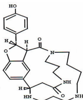
Aphelandrine ( C_{28}H_{36}N_4O_4 )
