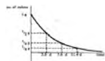
The exponential nature of radioactive decay curve
