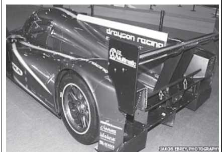
The Lola-Drayson electric car is an opportunity to test the structural batteries which will power some on-board systems. In this image a battery is indicated with yellow arrows.
