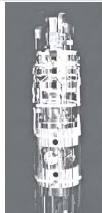
The NIST force sensor is a crystal of ions (charged atoms) trapped inside the upper region of the copper cylinder. A laser beam directed upward through the trap cools the ions. A force is applied in the form of an oscillating electric field, and a detector (not shown) measures the light reflected off the ions.
