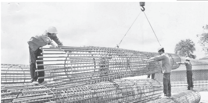
Steel fixing for construction of bole pile at Ayeyawady Bridge (Yadanatheinga) construction site.
