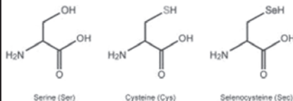
Comparison of selenocysteine (Sec) to the structurally similar amino acids serine (Ser) and cysteine (Cys).—INTERNET
