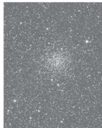
Image of the Galactic cluster NGC 6791, obtained using an Earth-based telescope. NGC 6791 is an extremely metal-rich and very old open cluster which has an abundant population of white dwarfs.
