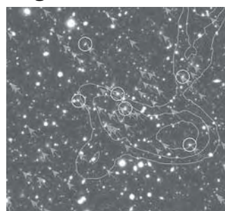
His false colour image is 3.4 arcmin on a side (about 1/10 the size of the moon). The arrows indicate galaxies that are likely located at the same distance, clustered around the centre of the image. —INTERNET
