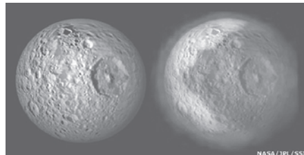
Mimas and a map of temperature variations that looks like Pac-Man.—INTERNET
