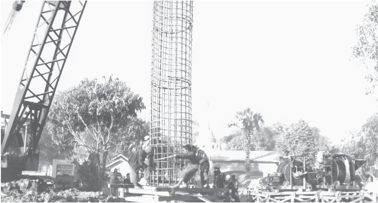
A heavy machinery unit driving RP 31 Bored Pile No (7) in Ayeyawady Bridge (Pakokku) project.
