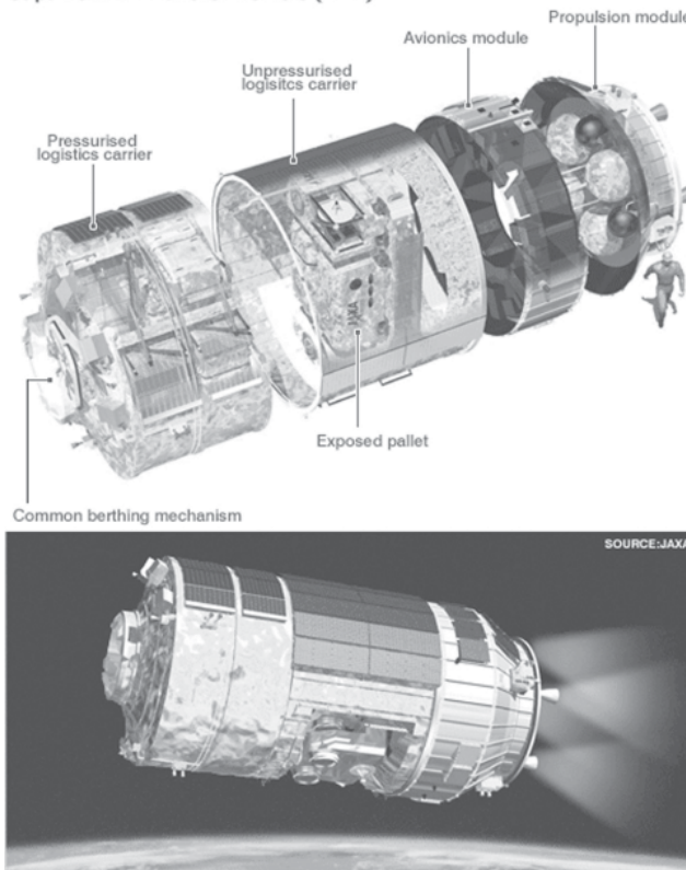
Japan's H-II Transfer Vehicle (HTV)
