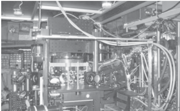
This is a strontium atomic clock operating at JILA, University of Colorado.
