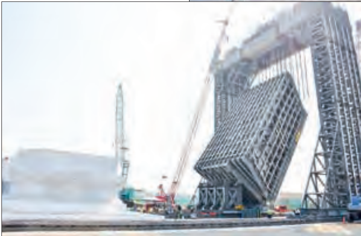
The lifting of the Maravijaya Buddha image is seen being 54.6° at noon on 28 January 2023.
