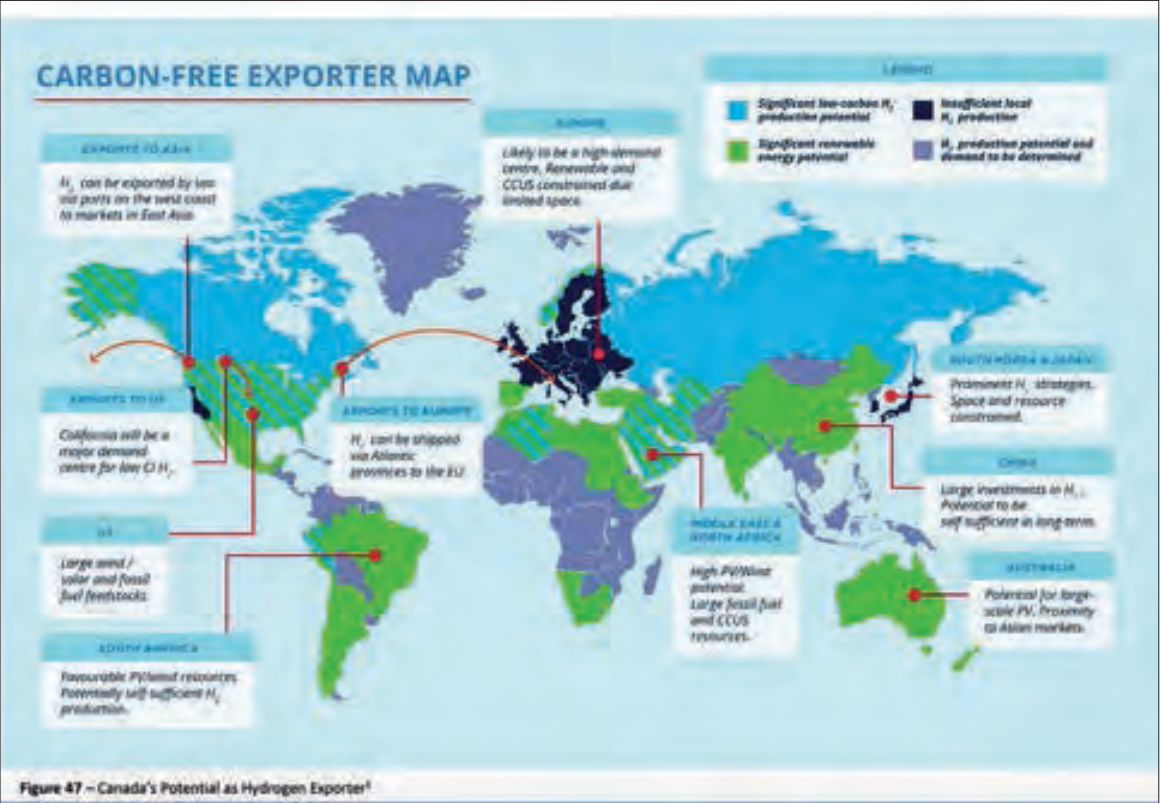
Regions and countries where the sun shines for long hours, such as the Middle East and Australia, are rich in green hydrogen. Source: Hydrogen Strategy for Canada, Based on data and maps from BloombergNEF Hydrogen Economy Outlook, March 2020 https://www.nrcan.gc.ca/sites/nrcan/files/environment/hydrogen/NRCan_Hydrogen-Strategy-Canada-na-en-v3.pdf (p.91)
