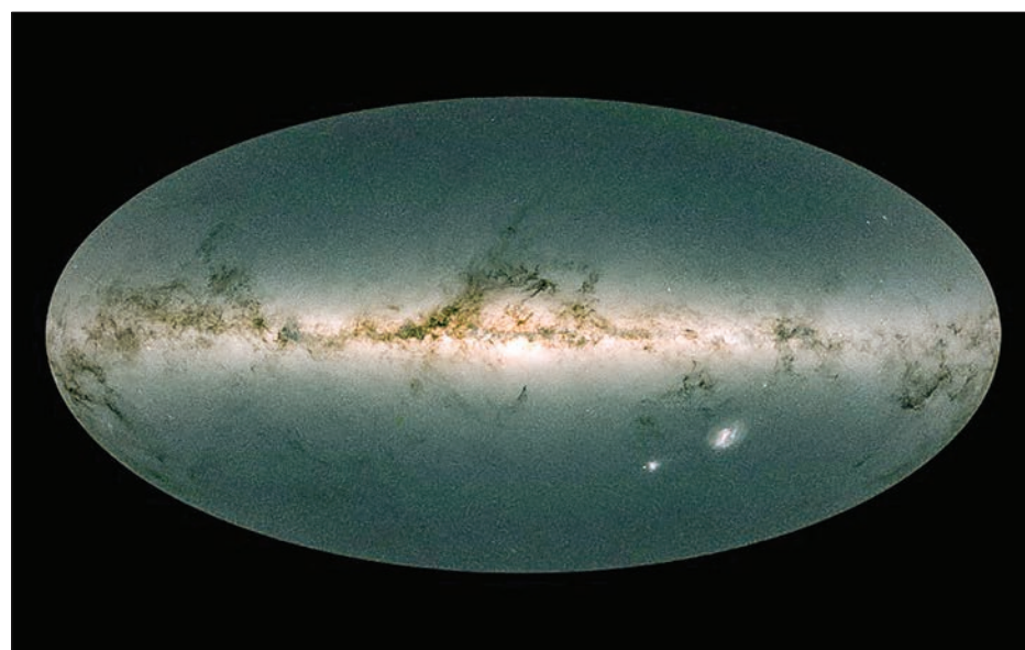
Pervious estimates put the mass of the Milky Way ranging between 500 billion and 3 trillion times the mass of the Sun. PHOTO: AFP
