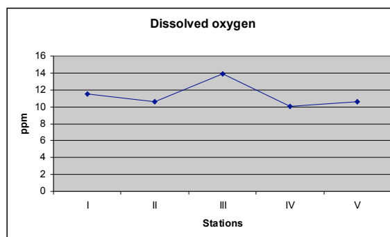
Fig. 6.1.5.4 Dissolved oxygen distribution along Pisa Dam environment.
