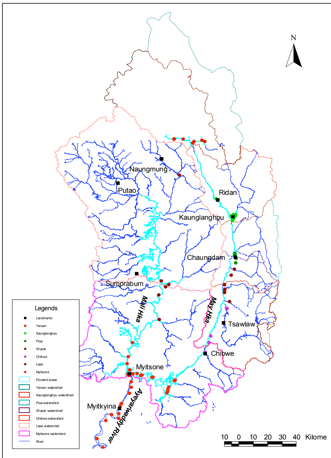
Fig. 4.1 (a). Sampling stations in the flood areas along May Hka, Mali Hka and Ayeyarwaddy Rivers.
