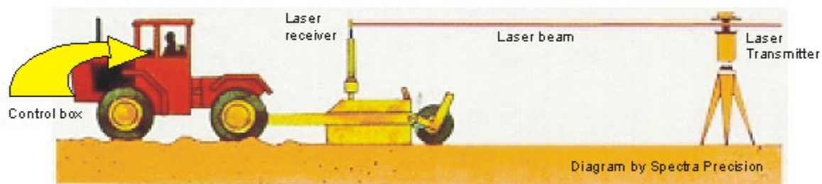
Figure 2. Schematic representation of laser leveling (IRRI: http://www.knowledgebank.irri.org/rkb/benefits-of-laser-leveling.html )
