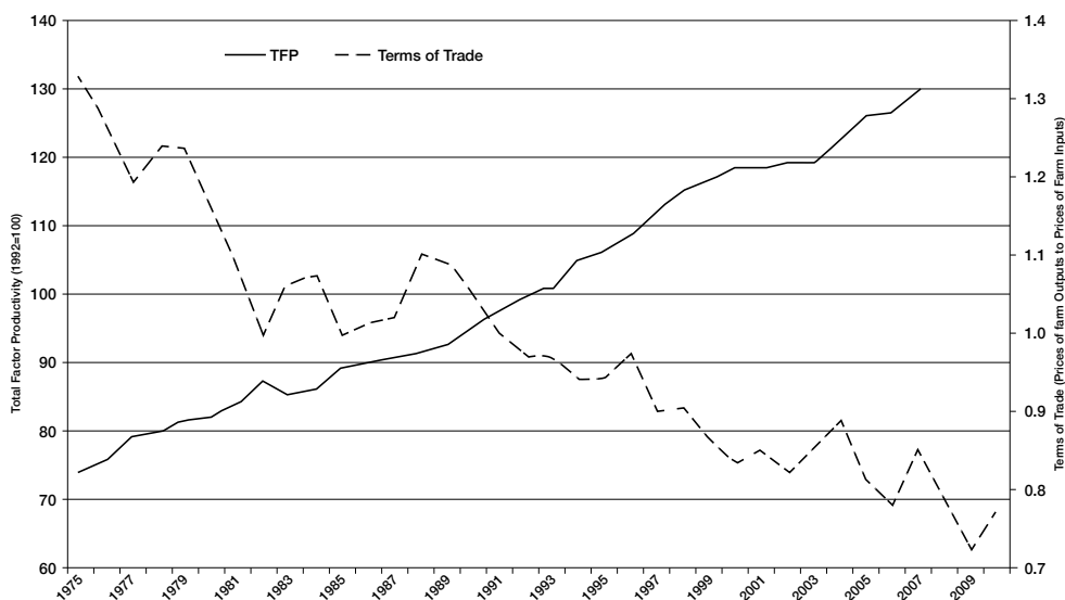
Figure 6: Higher TFP helped U.S. farmers compensate for declining ToT
